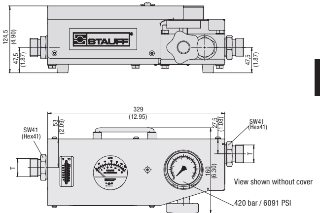
Dimensions SDMCR-750
